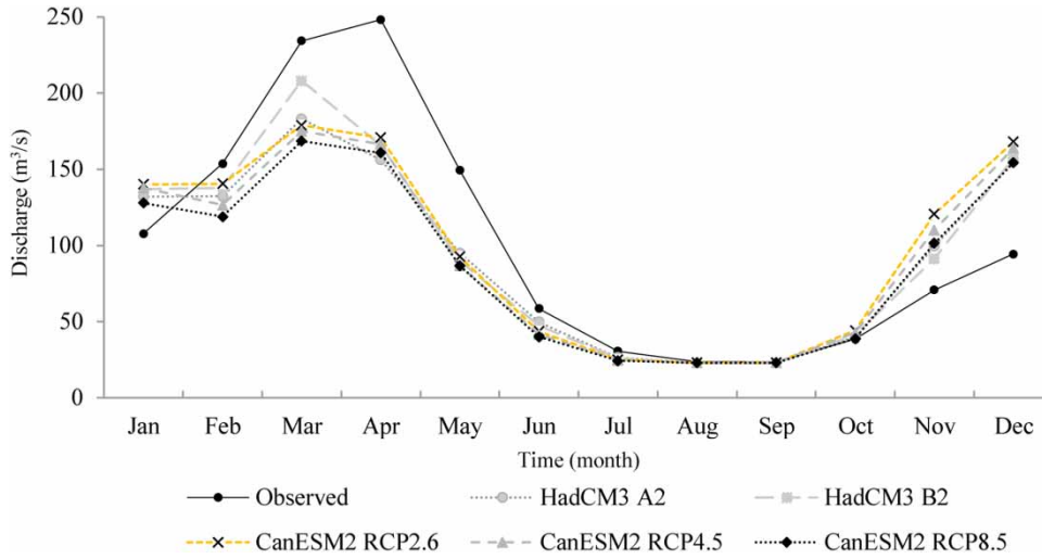
Figure 6 | The mean monthly inflow to Seimareh Dam in the 50-year observation and future periods.
