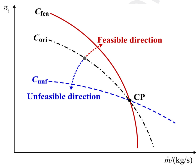
Figure 6 Illustration of optimization direction on one speed line.
