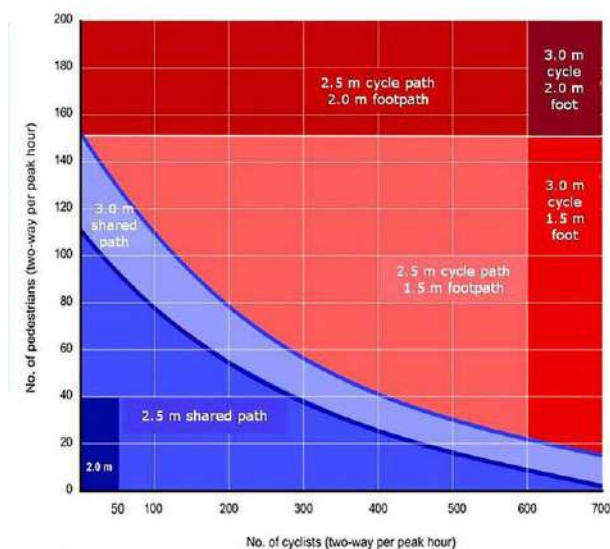
Fig 11: Diagram of the ranges of cross size for shared paths (blue and sky-blue) and separated pedestrian and cycle paths (red) with regard to their capacity to sustain two-way fluxes of pedestrians (ordinates) and cyclists (abscissas) - (Fowler, Lloyd, Munro, unknown year)
