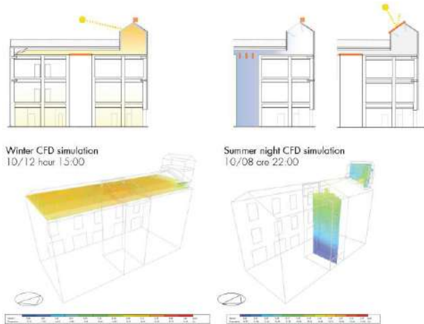
Fig.9: Solar chimney.
