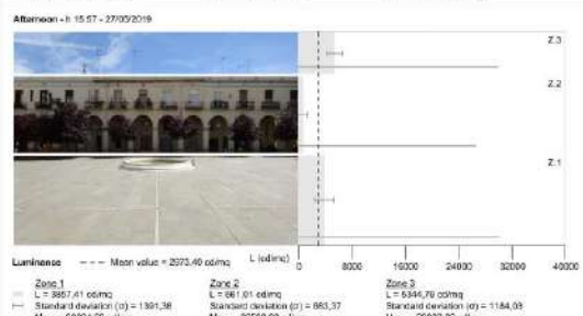
Fig. 5: The static analysis of natural lighting of the Plaza de Masadas . Graphic elaborations by the author
