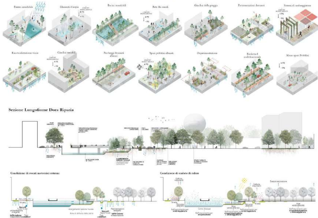
Fig. 7: Masterplan of the scenario proposed, composed by the systemic use of an Abacus of different blue and green actions and tactics, narrated through plants, figurative and functional sections representing the behaviour at possible climatic risk conditions.
