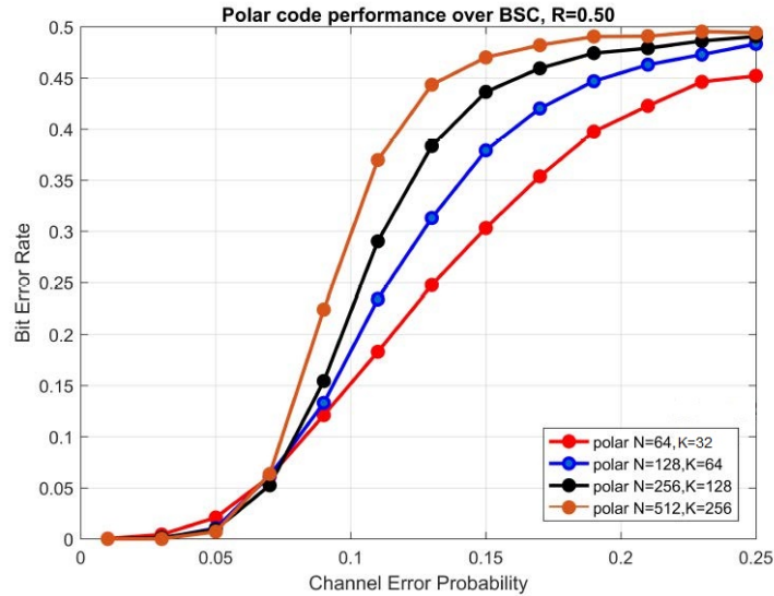
Figure 3. Performance of Non-Systematic Polar codes over a BSC channel for varying block sizes and rate R=K/N=0.5 .
