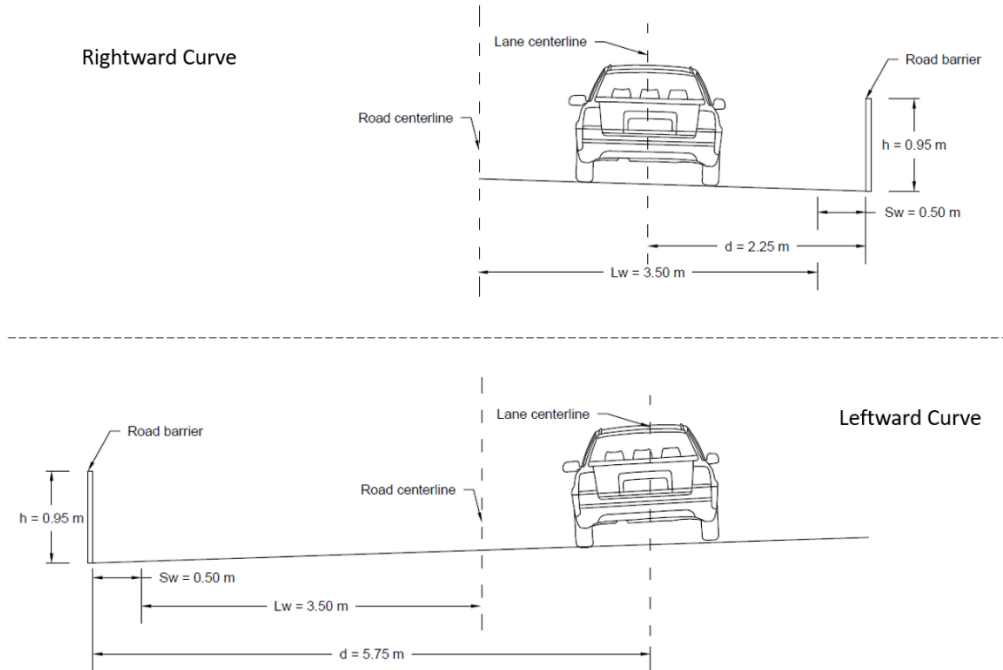
1 2 Figure 2 Cross-section of the roadway for RW and LW direction curves ( h = height of road barrier; 3 Lw = Lane Width; Sw = Shoulder Width; d = Distance from center of driving lane to the road 4 barrier).
