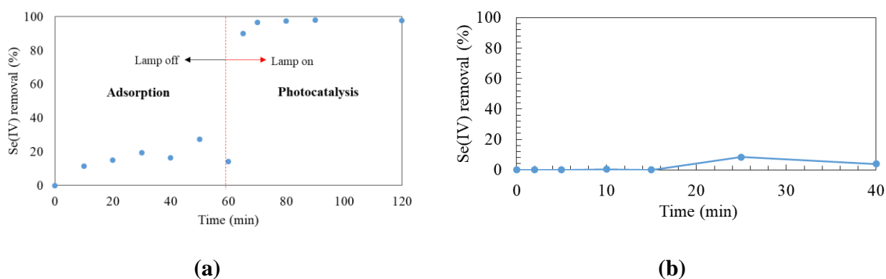
Figure S 19 – (a) Se(IV) removal (%) over time, with 60 min of adsorption in the dark followed by 60 min of photocatalysis. Photocatalyst \text{TiO}_2/\text{CoFe}_2\text{O}_4 produced using a TIPO/ \text{CoFe}_2\text{O}_4 mass ratio equal to 46.9 and calcined at 500 °C. Catalyst concentration = 0.1 g L -1 , pH = 3.5; and (b) Se (IV) removal (%) over time by photolysis, without the addition of catalyst and pH = 3.5.
