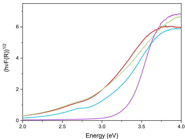
Figure 7. Tauc's plot applied to the undoped \text{TiO}_2 sample (purple line), \text{Fe}(3.5)\text{-TiO}_2 (green line), \text{Fe}(2.5)\text{-TiO}_2 (red line), and \text{Fe}(1.0)\text{-TiO}_2 (light blue line).
