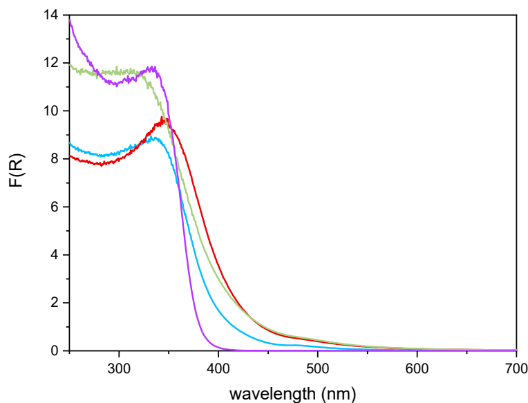
Figure 6. DR-UV-Vis spectra obtained with the undoped \text{TiO}_2 sample (purple line), \text{Fe}(3.5)\text{-TiO}_2 (green line), \text{Fe}(2.5)\text{-TiO}_2 (red line), \text{Fe}(1.0)\text{-TiO}_2 (light blue line).
