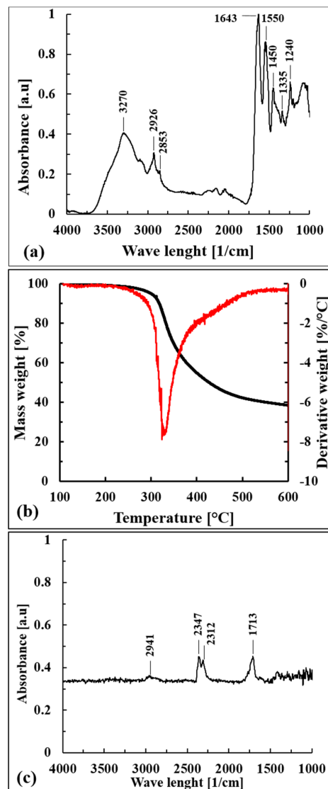
Figure 2. (a) ATR spectrum of WB fibers, (b) TGA and DTA curves of dried WB fibers, and (c) FT-IR spectrum of degradative products released by WB fibers at T_{peak} ( 328.6\text{ °C} ).
