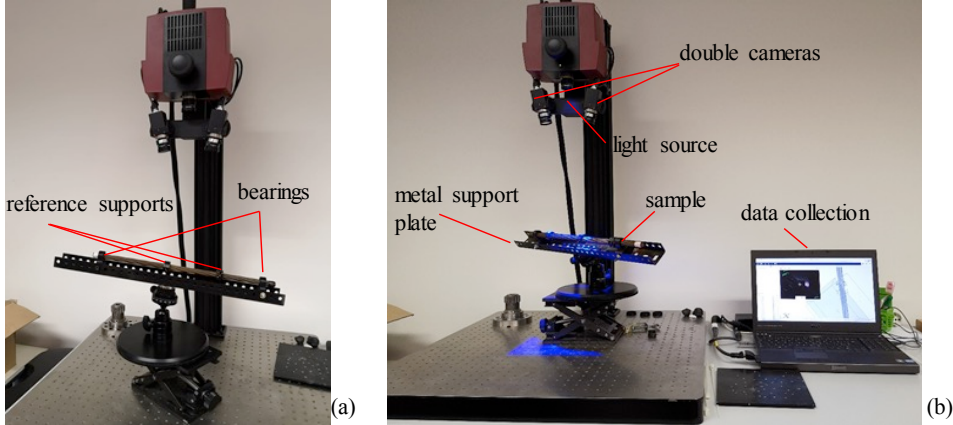
1 2 Figure 6. Structured light scanning system: (a) final configuration and (b) scanning phase.
