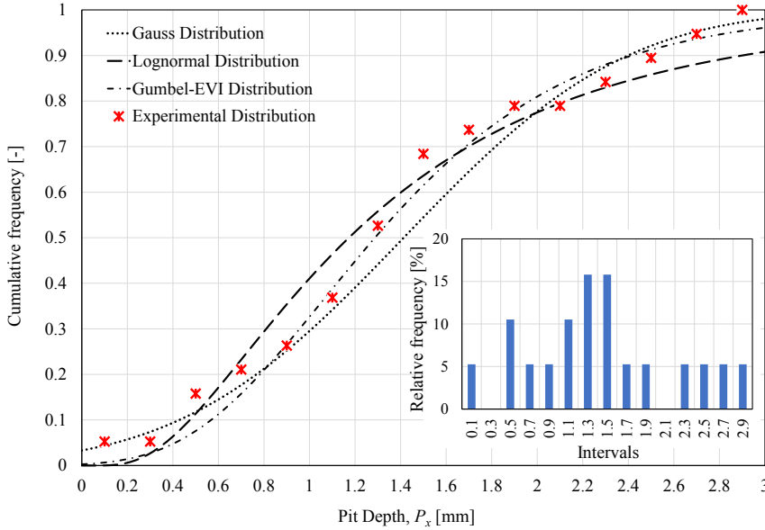
7 8 Figure 23. Statistical Investigation of maximum pit depth, P_x .
