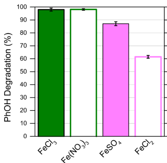
Figure 2.2.3 Phenol degradation resulting from the use of CS-Fe(III, II) complexes applied as homogeneous catalysts obtained with different iron salts (FeCl 3 , Fe(NO 3 ) 3 , FeSO 4 , FeCl 2 ). The reactions were performed with metal:PhOH:H 2 O 2 = 1:1:3 mass concentration ratio, and metal concentration as in Figure 2.2.1 a.
