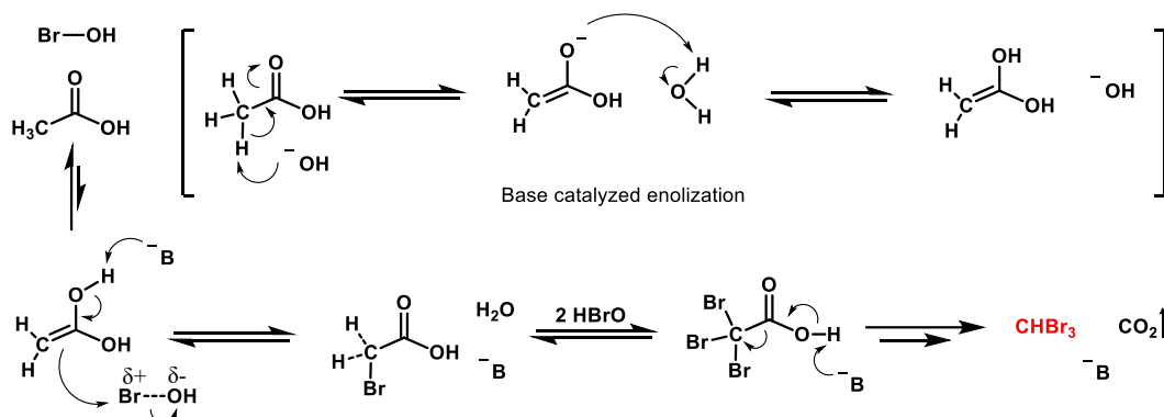
Figure 3.2.4 Rationalization of the possible reaction mechanism causing the formation of \text{CHBr}_3 in the presence of PAAM and \text{Br}^- . The proposed mechanism is based on the Hell-Volhard-Zelinsky reaction.
