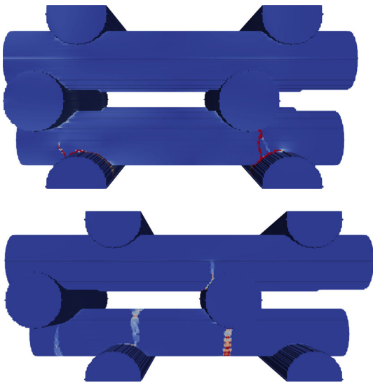
Fig. 5 Damage distribution for two different fiber shifting \alpha = 0.2 and \alpha = 0.4
