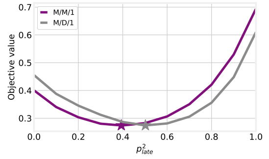
Fig. 7. Small-scale scenario for lane change: value of the objective (14) as a function of p_{late}^2 , when road segments are modeled as M/M/1 (purple) or M/D/1 (gray) queues.
