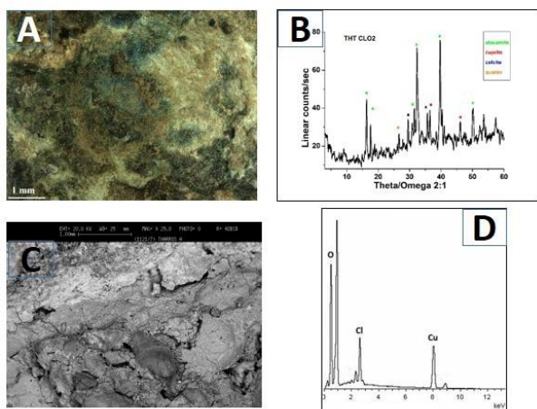
Figure 4. Coin THT CLO2: OM image (A), XRD spectrum (B), SEM image (C) and EDS spectrum (D).
