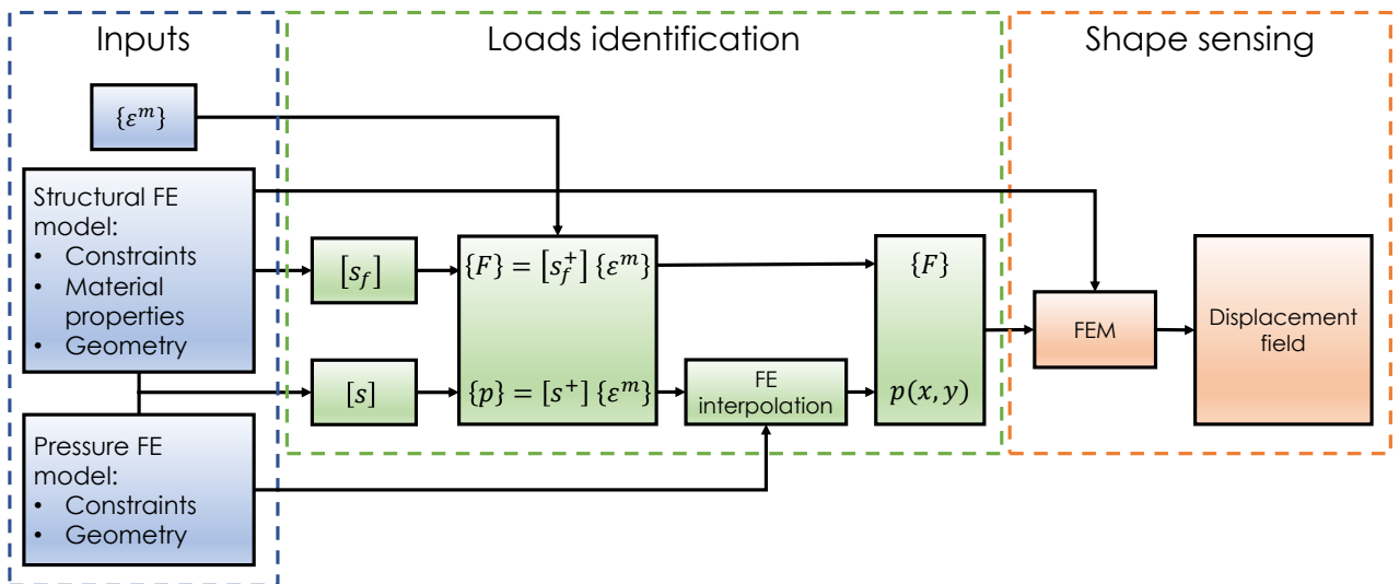
Figure 1: Loads identification and shape sensing integrated process - The inputs of the process are highlighted in blue. The load identification step is highlighted in green and the shape sensing step is highlighted in orange.
