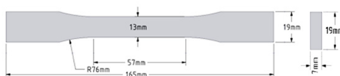
Fig. 1. Tensile test specimen's geometry and dimensions.
