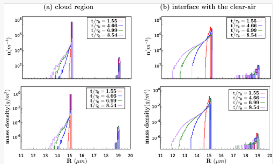
Water droplet size and mass distribution. Simulation of the monodisperse drop population centered around the initial value of 15 \mu\text{m} , 8 \cdot 10^6 droplets. Panel (a) droplet size distribution and mass distribution as a function of radius classes for the cloud region (HIT turbulence). Panel (b): droplet size distribution and mass distribution as a function of radius classes for the cloud and clear
