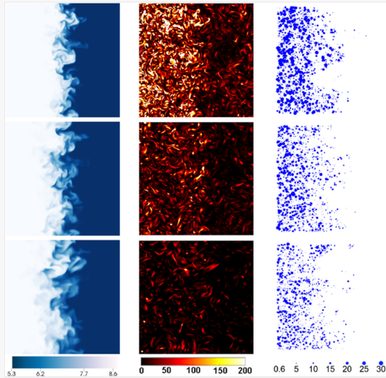
Visualization of fields inside the turbulent shearless layer in between the cloud and clear-air portions of the simulation: water vapor (left, legend values in \text{kg/m}^3 ), enstrophy (middle, values in \text{sec}^{-2} ) and droplets (right, diameters in arbitrary units, polydisperse population). From top to bottom, snapshots at 3, 6 and 9 eddy turnover times.
