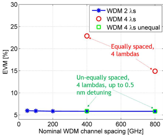
Fig. 5. EVM as a function of the nominal WDM channel spacing for different WDM transmission scenarios. An OPL of 21 dB is considered.
