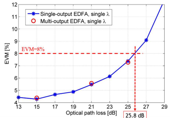
Fig. 4. EVM as a function of OPL for single-wavelength transmission using a single-output or a multi-output EDFA.
