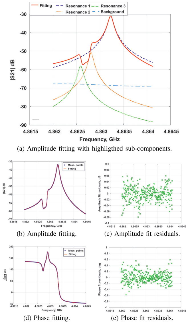
FIGURE 8. Detailed fitting results of the triplet in Fig. 7.
