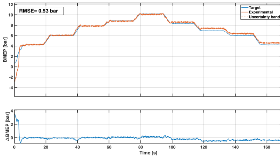
(a) Controller disabled
