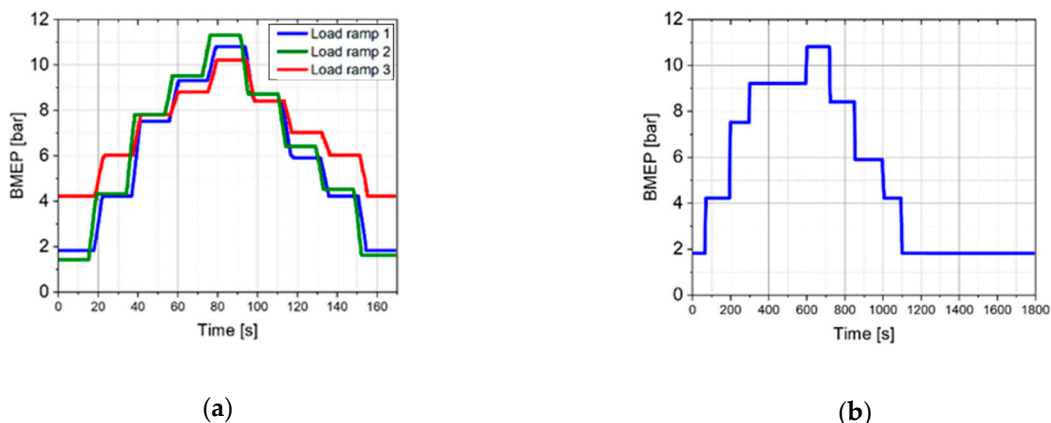
Figure 4. (a) BMEP variation over time for the baseline load ramps #1, #2, #3. The initial coolant temperature was around 65 °C over the three ramps; and, (b) BMEP variation for the load ramp test #4, that was a repetition of load ramp #1 with longer stabilization time after each load variation, and an initial coolant temperature of around 85 °C.
