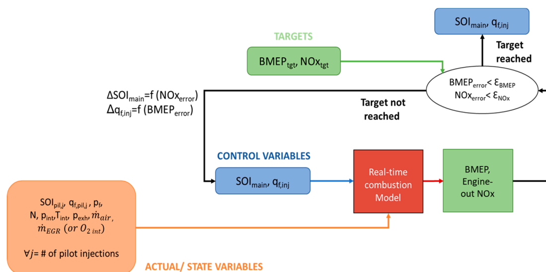
Figure 5. Conceptual scheme of the controller.
