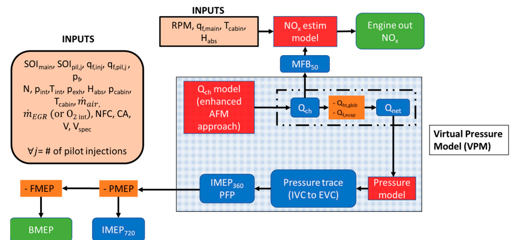
Figure 6. Scheme of the combustion model.
