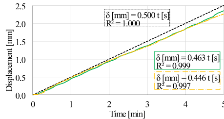
Figure 4: Uni-axial test nominal elongation ramp imposed at the UTM crosshead (dotted line, black) and actual elongation rate, as measured by DIC, for G-ER (solid, green) and G-EW (dash-dotted, yellow) specimen groups. Linear fitting expressions are also given alongside the coefficient of determination R^2
