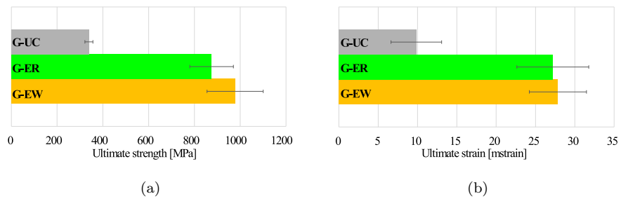
Figure 13: Mean ultimate stress (a) and mean ultimate strain (b) evaluated in uni-axial traction for all specimen groups
