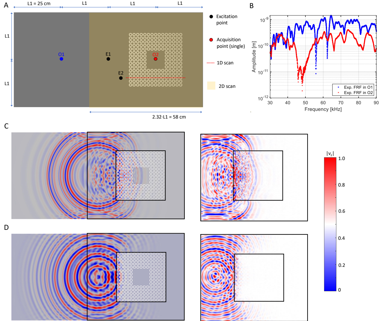
Figure 3: (A) Schematic representation of the FE model used for the three-dimensional transient dynamic computation. The specimen consists of a PMMA rectangular plate of length 4 \cdot L1 = 1000 mm, width 2 \cdot L1 = 500 mm and height H = A = 19 mm), where 200 unit cells have been drilled in the shape of a square ring. Excitation points are highlighted as black dots. Measurements are performed through Scanning Laser Doppler Vibrometry in specific points outside (blue dot named O1 ) and inside (red dot named O2 ) the phononic ring, along a 1D line scan (dotted red line), and in a 2D region scan (orange rectangle superimposed to the schematics of the plate). (B) Frequency Response Function (FRF) of the system in the O1 and O2 measurement points, both located at L1 from the E1 excitation point. A clear drop in the amplitude is visible in the frequency domain for the measurement inside the phononic region. Numerical (left panel) and experimental (right panel) full wavefield reconstructions of the out-of-plane velocity for a (C) 2 and a (D) 21 sine cycles centered at 50 kHz Hann windowed excitation signals fed in E1 . A color map of the out-of plane velocity is reported on the right, and normalized with respect to the maximum displacement.
