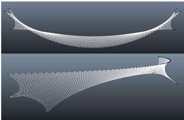
Figure 13: Form-finding of the shell of the curved shell-supported footbridge using a Particle Spring System
