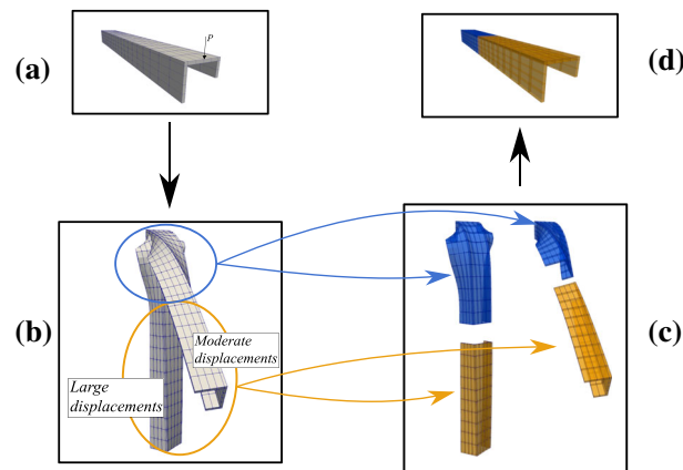
Fig. 4 Logical steps to perform the geometrically nonlinear analysis using the NDK approach
