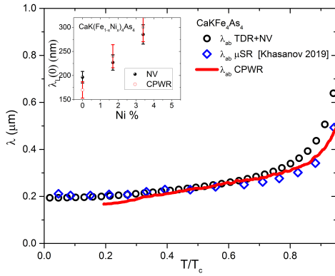
Fig. 3. Comparison of the \lambda_L measurement results from different technique on the same material ( \text{CaK}(\text{Fe},\text{Ni})_4\text{As}_4 ). TDR and NV data from [14], \mu\text{SR} data from [17].
