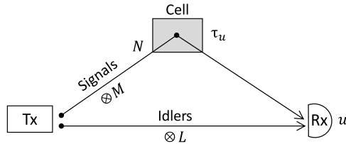
Fig. 1. Quantum reading of a memory cell. A memory cell encodes a bit u in a lossy channel with transmissivity \tau_u . The cell is read by a transmitter (Tx), which irradiates M signal modes and N mean total photons over the cell, plus extra L idler modes sent to the output. The receiver (Rx) performs a generally joint measurement of signals and idlers, decoding the bit u up to some error probability p_{\text{err}} . Quantum reading corresponds to using a quantum source of light for the Tx so that we outperform any classical source in the readout of the bit. The scheme can be realized in reflection or in transmission, as done in our experiment.
