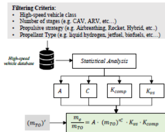
Fig. 5: Algorithm for the estimation of the ratio between Operative Empty Mass and the Take Off Mass
