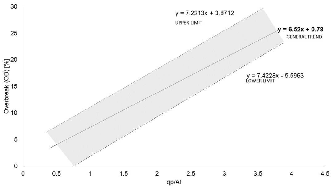
Figure 13- Trend of the observed over-break as a function of the ratio qp/af (from data by Verma et al., 2018).
