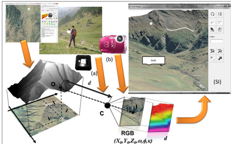
Figure 7 - The generation of SI using STOP data (b) with and (a) without additional digital camera.
