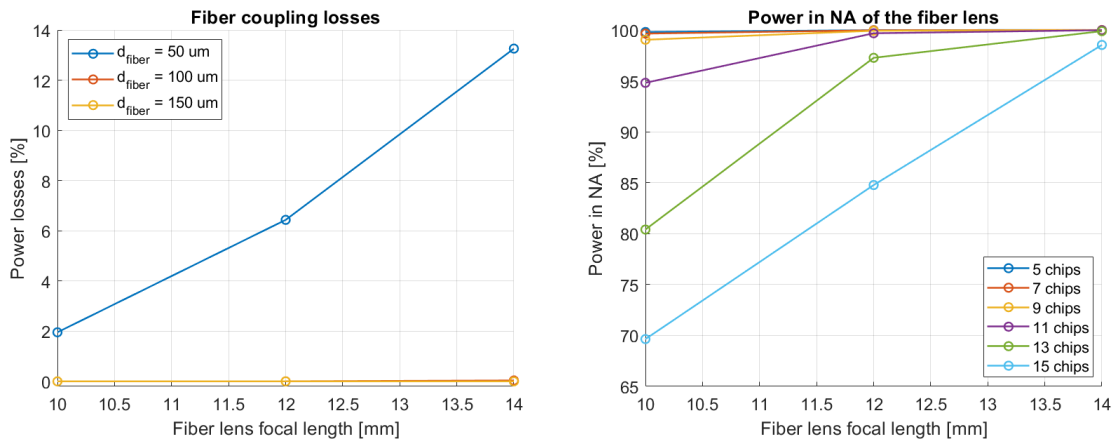
Figure 3. Effects on focal length of the collecting lens on the NA of the output beam and on fiber coupling losses.
