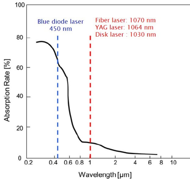
Figure 1. Absorption rate in copper for different wavelengths.
