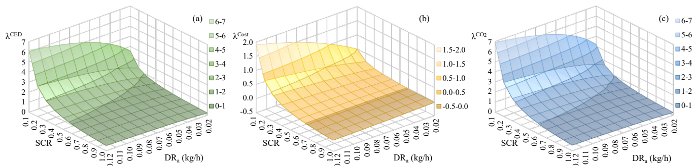
Fig. 2. Breakeven surfaces for (a) CED, (b) Cost and (c) CO 2 emissions.
