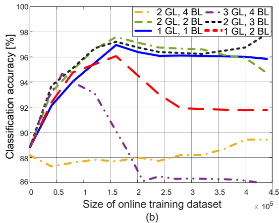
Fig. 10. Effect of the number and quality of labels on the obtained classification accuracy, for a varying size of the online training set: (a) LS algorithm and (b) RLS. For the ego vehicle, the availability of 3 good-quality labels and 4 bad-quality labels is considered.
