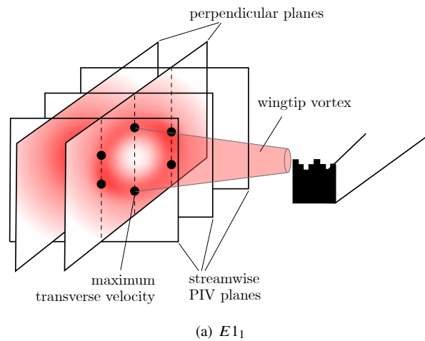
Fig. 13 Schematic illustration of how (U_{tmax})_{av}/U_\infty is calculated.
