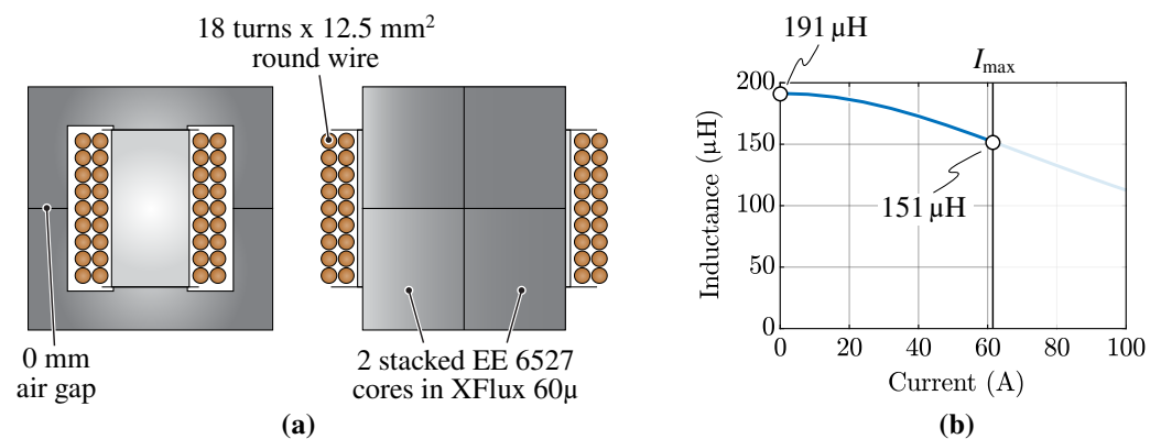
Figure 12. Schematic representation of the designed inductor ( L = L_f ) (a) and differential inductance value dependence on the DC-bias current (b), which highlights the soft saturation characteristic of the selected powder core material.
