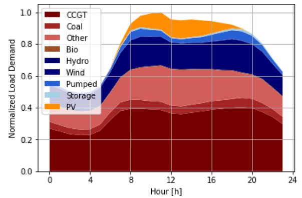
Fig. 4. Normalized load demand, not considering cross border imports.
