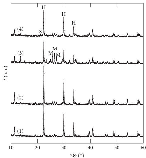
FIGURE 2: XRD patterns of powder-like samples 1, 2, 3, and 4 thermally treated at 1000°C for 5 hours (M = monoclinic celtsian, H = hexacelsian, S = sodium aluminosilicate).
