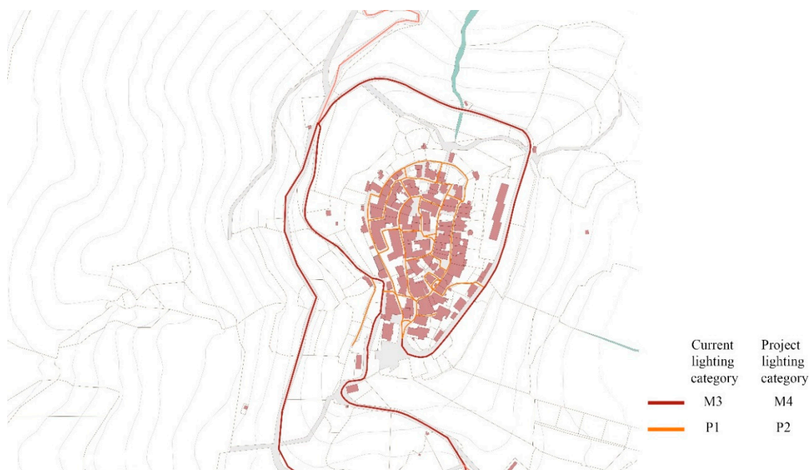
Figure 9. Road lighting classes (ex-ante and ex-post).
