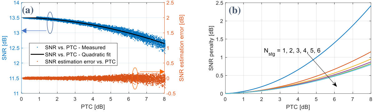
Fig. 1 (a): Results of the Monte-Carlo simulations as SNR as a function of the PTC. Number of stages: N_{stg} = 4 . (b): Parabolic fit of the SNR penalty as a function of the PTC with different number of stages (each emulating a WSS).
