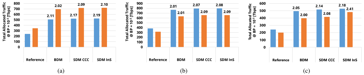
Fig. 4: Total Allocated Traffic at BP = 10^{-3} [Tbps] for reference case and upgrade solutions with uniform connection requests joint PDF (blue), population-based non-uniform connection requests joint PDF (orange) for (a) German, (b) US-NET and (c) COST topologies. Labels on top of the upgrade solutions bars are the corresponding traffic multiplicative factors with respect to reference case.
