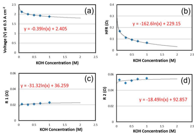
Figure 5. Logarithmic relationship of a) voltage at current density of 0.5 \text{ A cm}^{-2} , b) HFR or ohmic resistance originating from membrane resistance, c) R1 originating from HER and d) R2 originating from OER versus the different KOH concentration.
