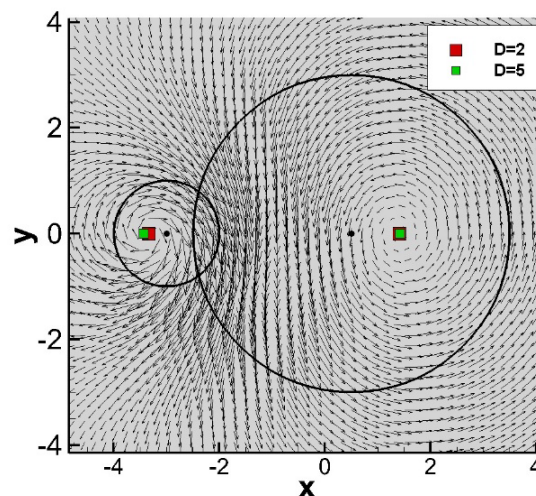
Figure 16. Case 5: r_{c2} = 3r_{c1}, \gamma_2 = -2\gamma_1, d < r_1 + r_2 .
