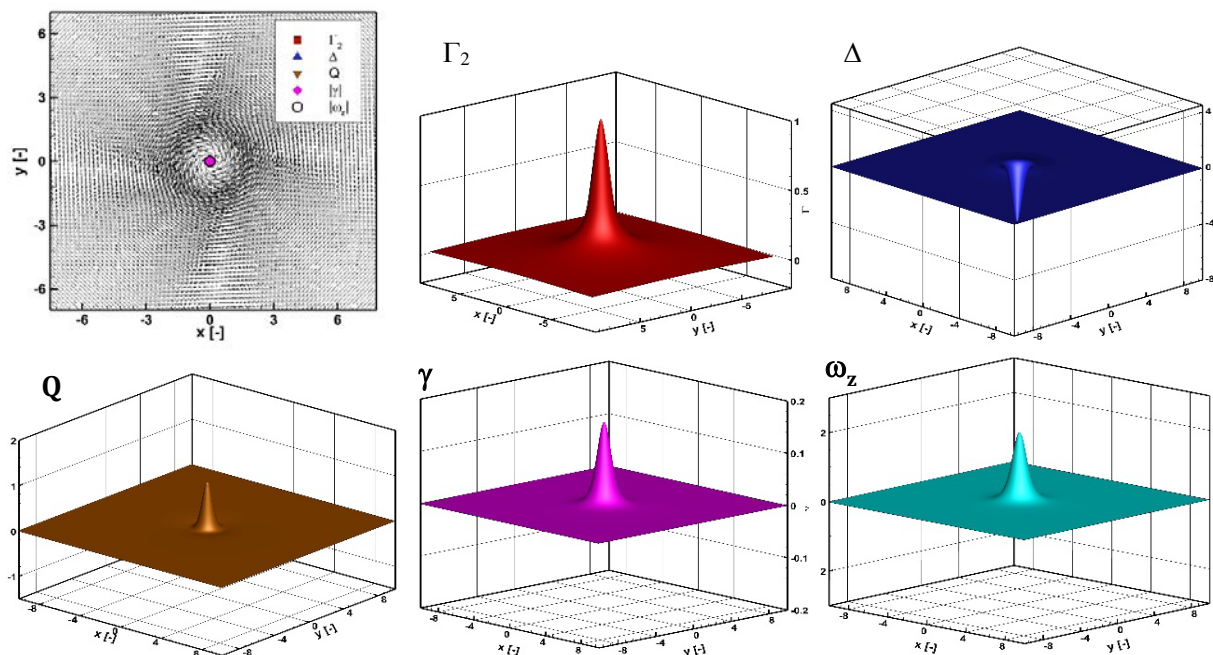
Figure 6. Vatisitas Vortex - Velocity field and detected centres with different criteria: Noise 0%.
