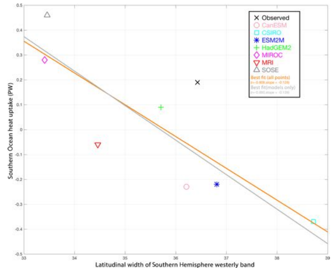
Figure 28. Scatter plot of the width of the Southern Hemisphere westerly wind band (in degrees of latitude) against the annual-mean integrated heat uptake south of 30^{\circ} S (in petawatts, PW – negative uptake is heat lost from the ocean), along with the “best fit” linear relationship for the models and observations shown. Enhanced from figure produced by recipe_russell18jgr.yml ; see Sect. 3.3.2. For further discussion of this figure, see the original in Russell et al. (2018). The calculation of the “observed” heat flux into the Southern Ocean is described in the text. The correlation is significant above the 98 % level based on a simple t test.
