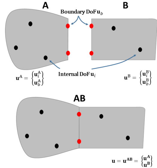
FIGURE 1. The FBS coupling: the two substructures A and B are coupled at their respective boundary DoF with rigid connections.
