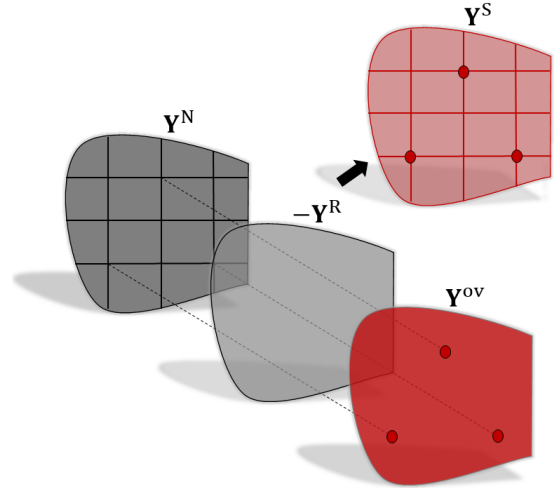
FIGURE 2. Equivalent models of the substructure A of Fig. 1: The parent numerical model \mathbf{Y}^N has the essential DoF. Its own dynamics are decoupled by the removed model \mathbf{Y}^R and coupled by \mathbf{Y}^{ov} . The resulting hybrid or expanded model \mathbf{Y}^S mimics at the corresponding overlay model's DoF.
