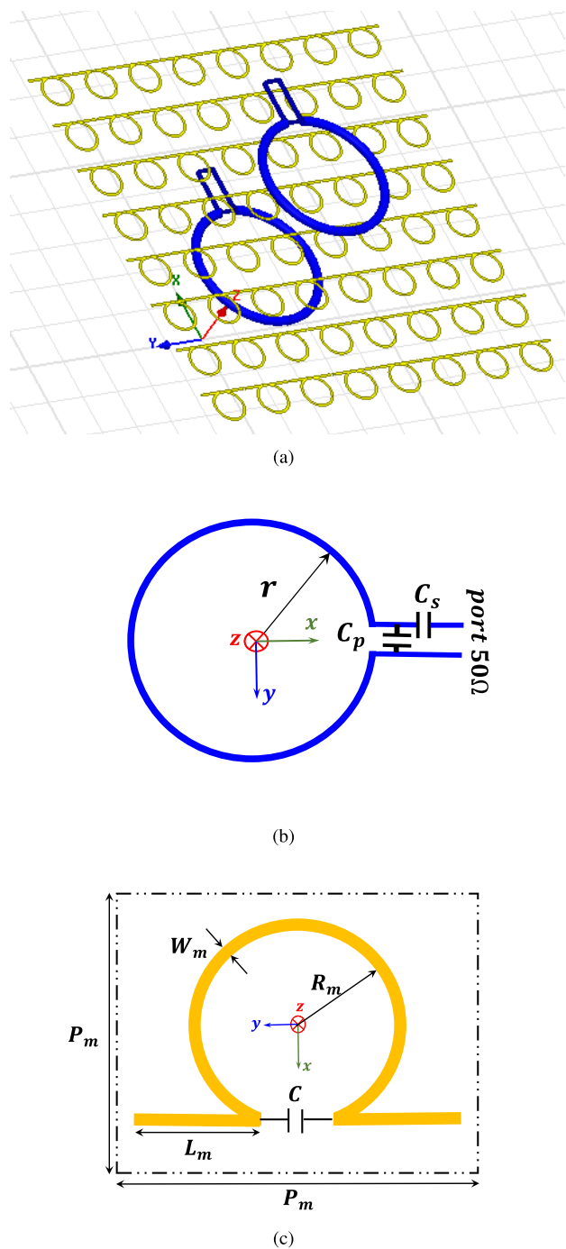
FIGURE 5. (a) Configuration of the proposed HMS-assisted WPT system including two resonators and an HMS positioned between them, (b) sketch of the transmitter(receiver) resonator, and (c) sketch of the Omega-type particle forming the desired HMS.
