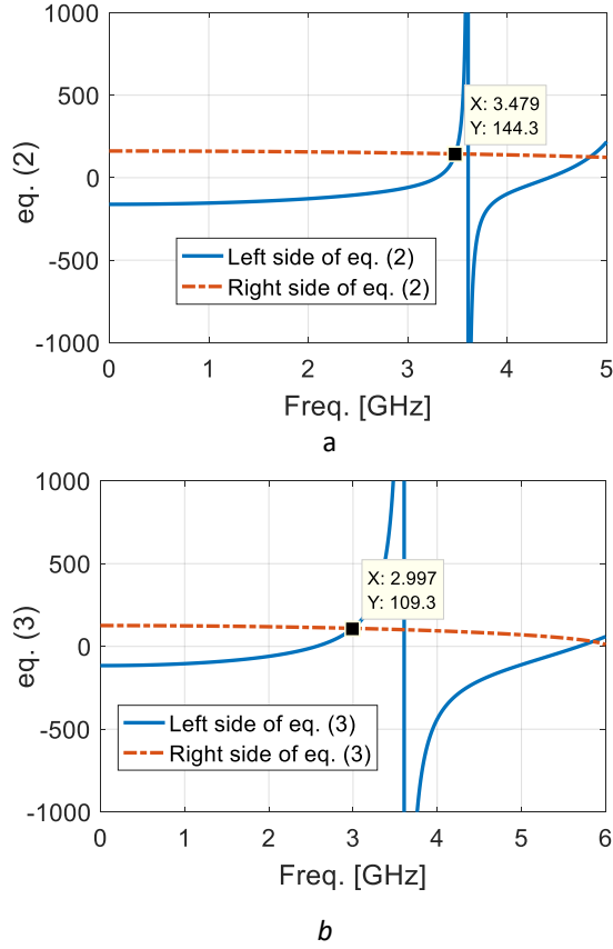
Figure 9. The graphical solution for the resonant frequencies of the DRA, (a) TE_{111}^x mode, (b) TE_{111}^y mode.
