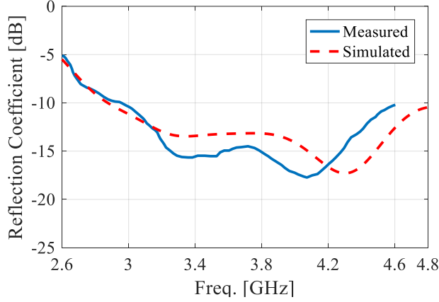
Figure 2. The measured and simulated input scattering parameter, |S_{11}| , of the proposed DRA.
