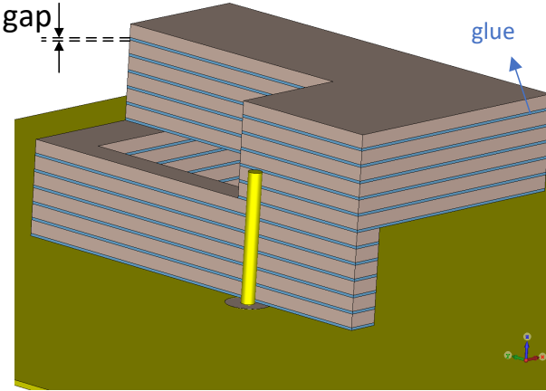
Figure 3. The perspective view of the DRA.
