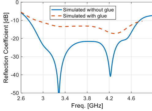
Figure 4. The simulated reflection coefficient of the antenna with and without the adhesive material between the layers, gap = 0.1 mm.
