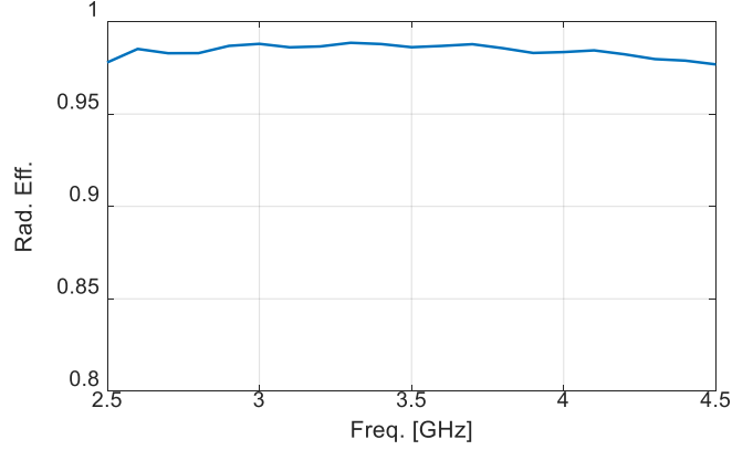
Figure 11. The simulated radiation efficiency of the proposed antenna.
