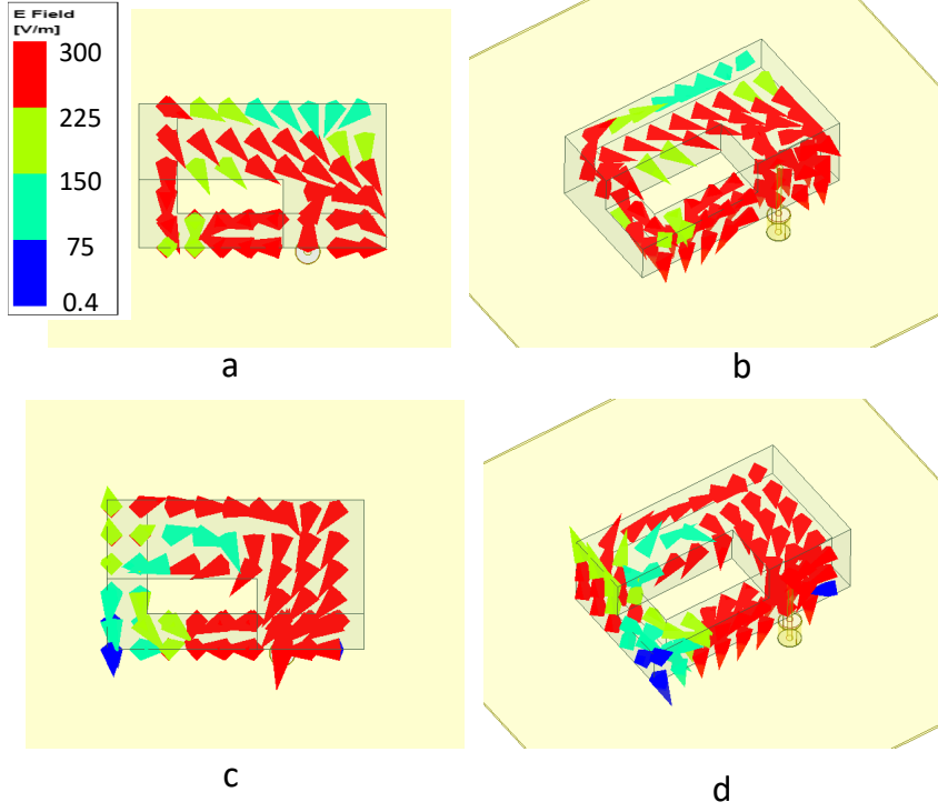
Figure 8. The Electric field distribution of the proposed antenna at 3.7GHz. (a) -45^\circ , top view (b) -45^\circ , 3D view (c) 45^\circ , top view (d) 45^\circ , 3D view.
