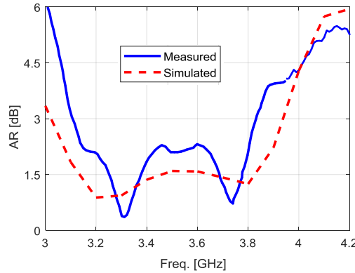
Figure 5. The measured and simulated axial ratio (AR) of the antenna.
