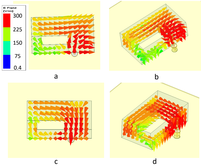
Figure 7. The Electric field distribution of the proposed antenna at 3.3GHz. (a) TE_{111}^x mode, -45^\circ , top view (b) TE_{111}^x mode, -45^\circ , 3D view (c) TE_{111}^y mode, 45^\circ , top view (d) TE_{111}^y mode, 45^\circ , 3D view.
