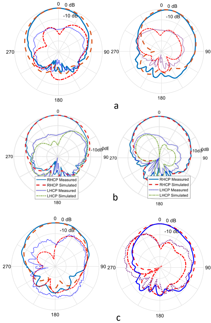
Figure 10. The measured and simulated results of the radiation patterns (a) at 3.2 GHz, (b) at 3.5 GHz, (c) at 3.8 GHz. Left: XZ plane ( \phi=0 ), Right: YZ plane ( \phi=90 ).
