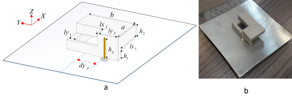
Figure 1. The configuration of the proposed DRA. (a) 3D view (b) the fabricated prototype.
