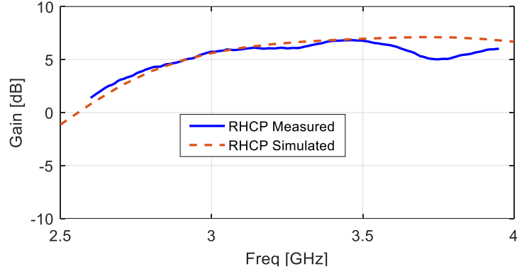
Figure 6. The measured and simulated RHCP gains of the antenna.
