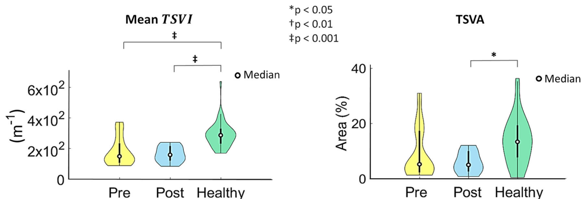
FIGURE 4. Violin plots of the mean value of the Topological Shear Variation Index ( TSVI ) and the Topological Shear Variation Area ( TSVA ) in the bifurcation region (delimited by sections CCA3-ICA5-ECA2) for pre-CEA (Pre), post-CEA (Post) and healthy cohorts. The distribution, median and quartile range are displayed for each cohort. Differences among the three cohorts are evaluated with a Wilcoxon signed-rank test.
