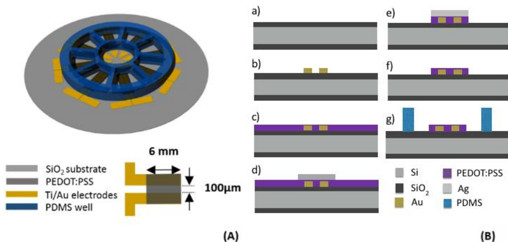
Figure 1. (A) Organic electrochemical transistor (OECT) layout. (B) Device fabrication process: (a) \text{SiO}_2 substrate, (b) patterned electrical contacts, (c) poly(3,4-ethylenedioxythiophene):polystyrene sulfonate (PEDOT:PSS) film, (d) Ag layer, (e) excess of PEDOT:PSS removed by \text{O}_2 plasma, (f) Ag removal by E6 wet etching, and (g) bonding of poly(dimethylsiloxane) (PDMS) well.
