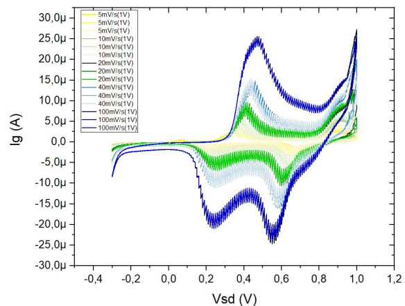
Figure 3 60I OMD's hysteresis: response of the I_g current to V_{SD} sweeps.
