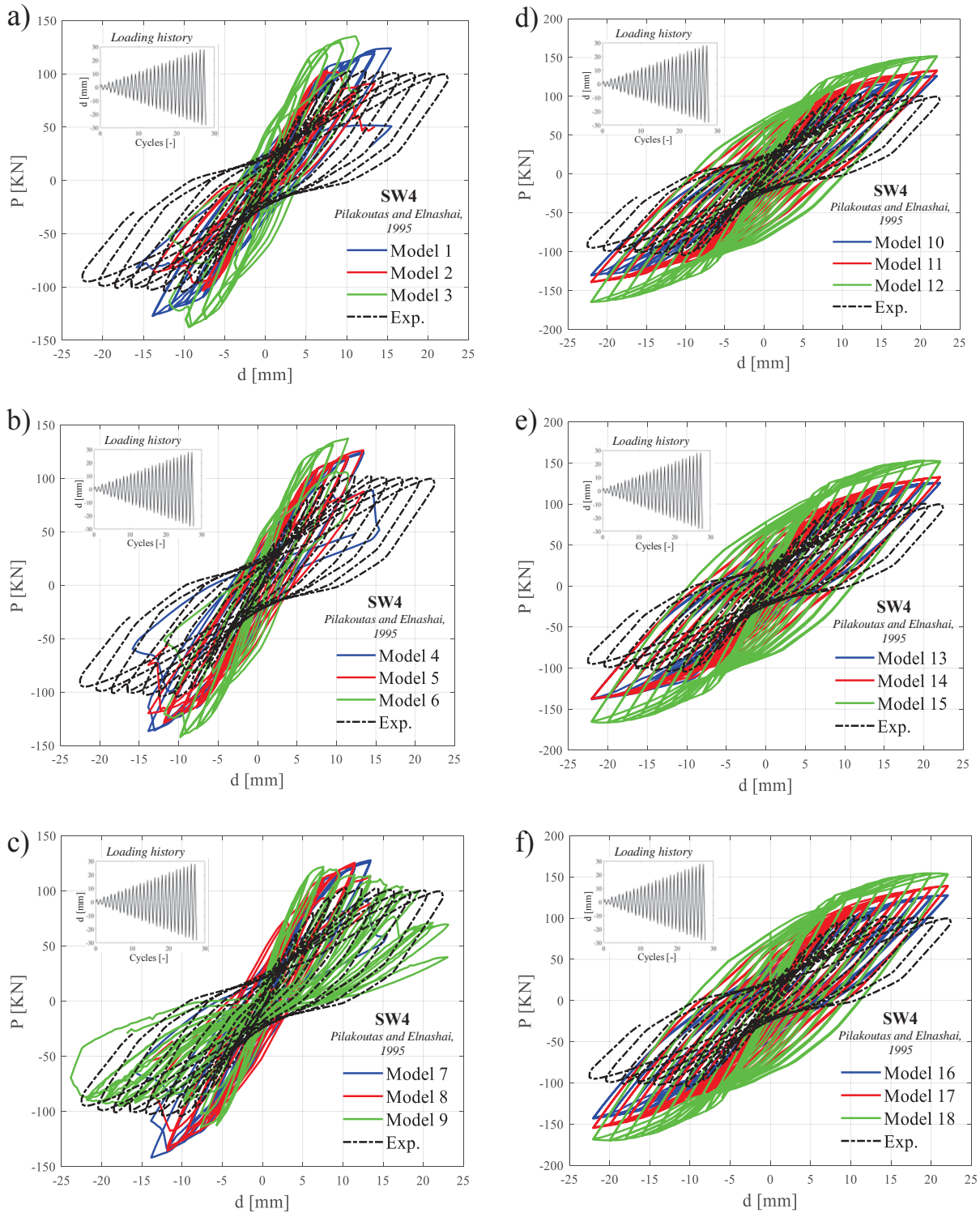
Figure 2: Comparison between NLFEMs and experimental tests expressed as load vs displacement curves - SW4 of [19]; (a-c) Numerical code A, (d-f) Numerical code B.
