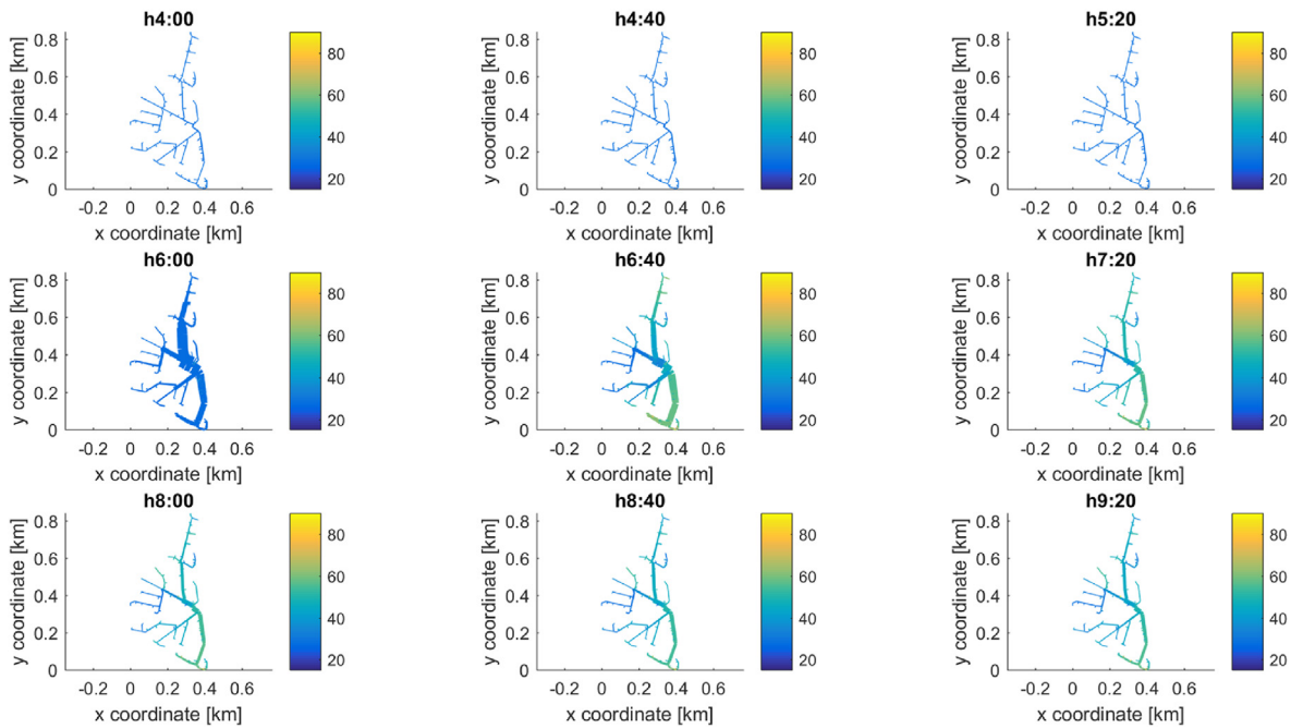
Fig. 6. Snapshots of temperature of water in the pipelines for different time. The depth of the lines is proportional to the mass flow rates flowing.
