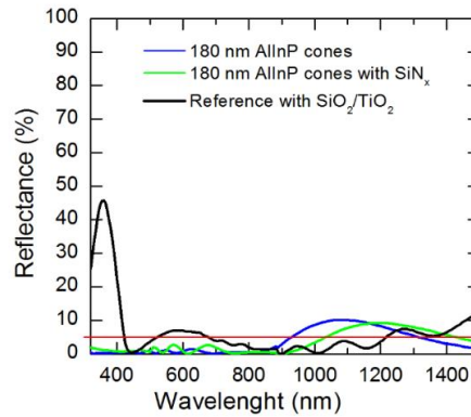
Fig. 29 Reflectance results of 180 nm AlInP cone structure. The red line represents the 5 % reflectance.
